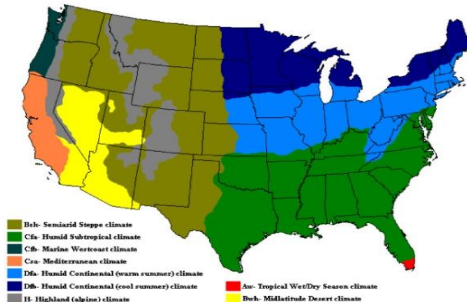
Climate Zones of the Continental United States
